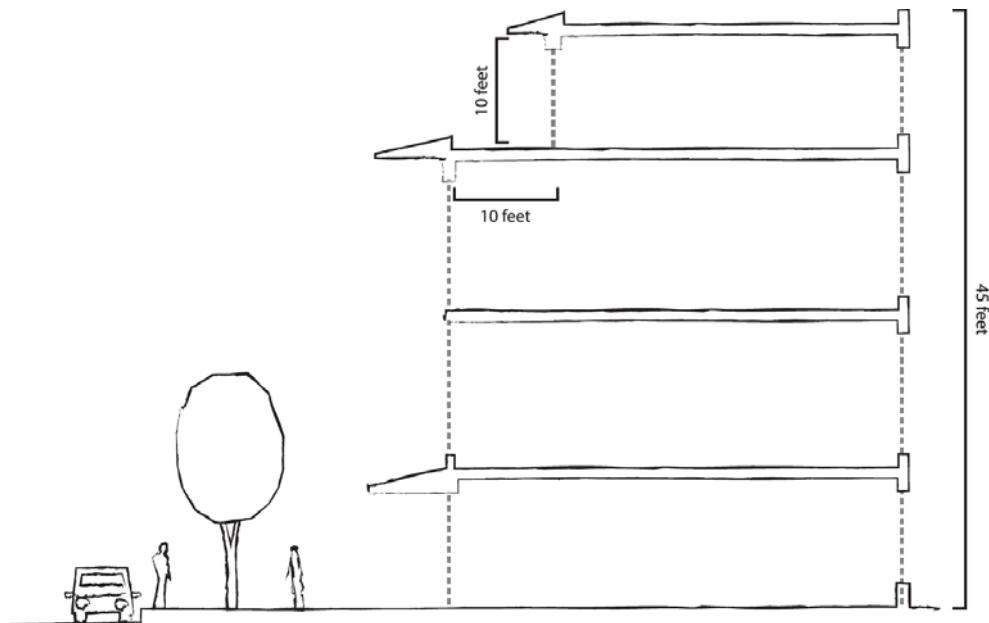
Illustration 1: Top Floor Setback
