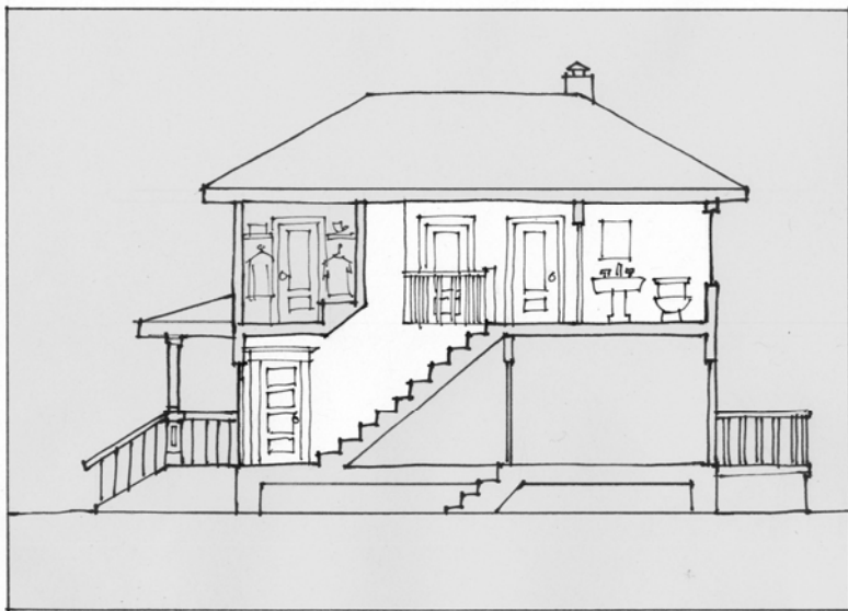
Figure 2: Above Grade Secondary Suite
