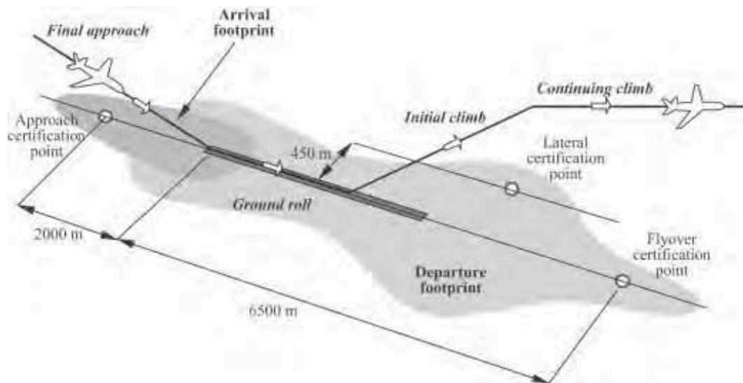
Figure 5: Illustration of how an aircraft noise footprint is determined with the different approach and departure stages at certification stages. The single event energy summation of different aircraft noise footprint over a period result in the forecasted noise contours.
