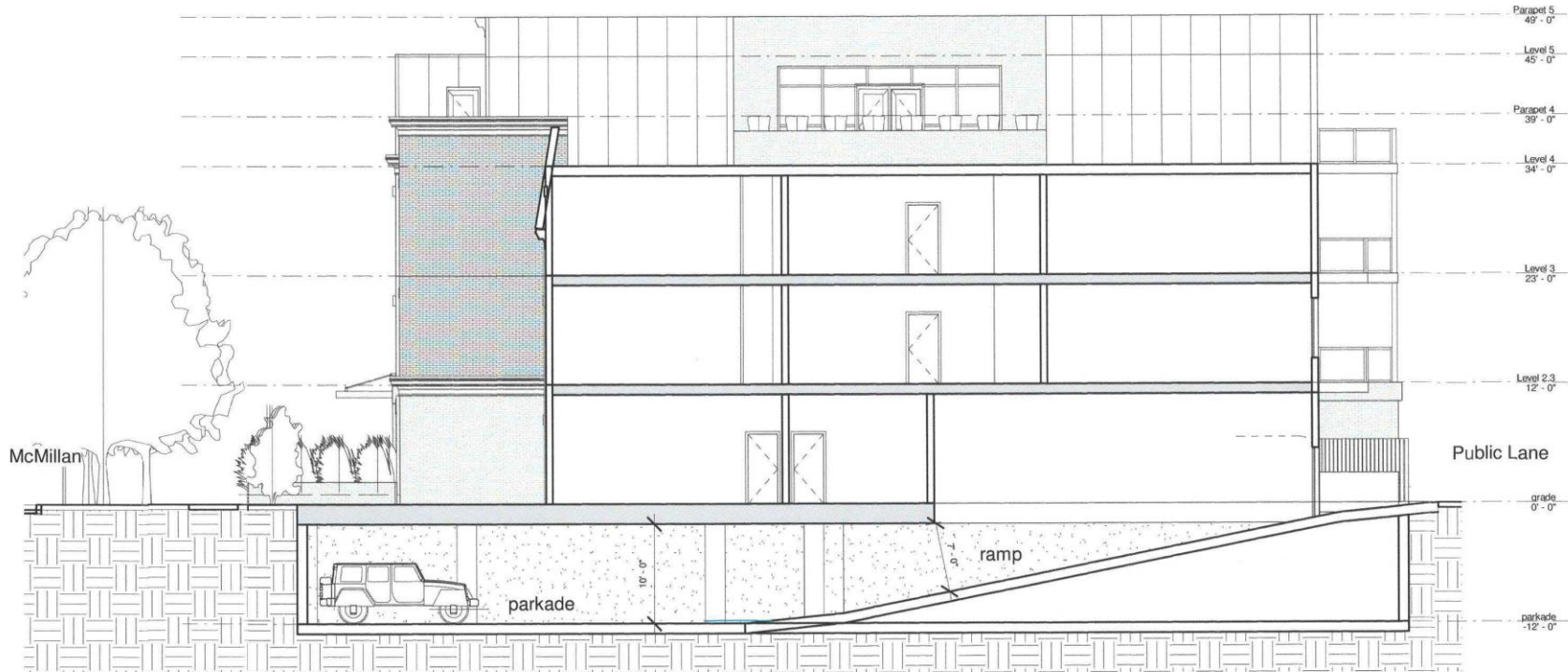
① Section 1 3/32" = 1'-0"
