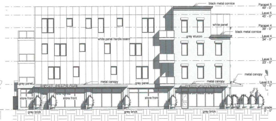
② West 1/16" = 1'-0"
