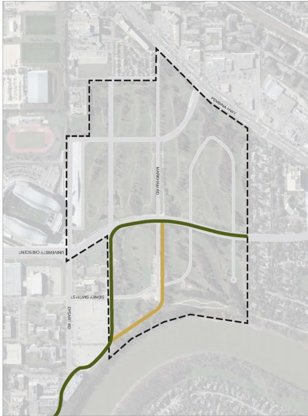
STAGE 1 PROPOSED RELOCATION
