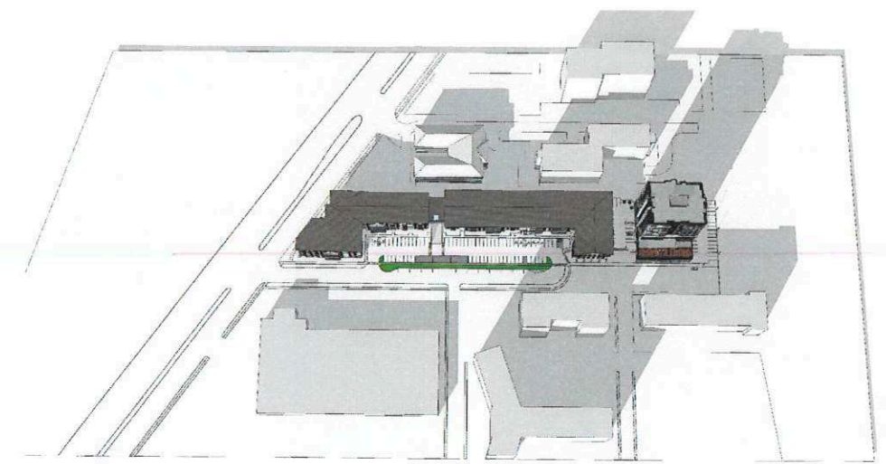
Pembina Tower, Winnipeg- Shadow Study- GMT -0600 22nd September- 03PM
