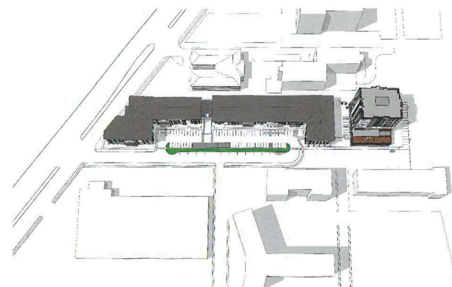
Pembina Tower, Winnipeg- Shadow Study- GMT -0600 21st June- 03PM
