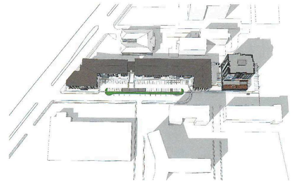
Pembina Tower, Winnipeg- Shadow Study- GMT -0600 22nd September- 03PM
