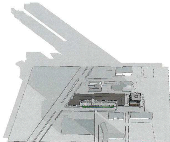
Pembina Tower, Winnipeg- Shadow Study- GMT -0600 22nd September- 09AM
