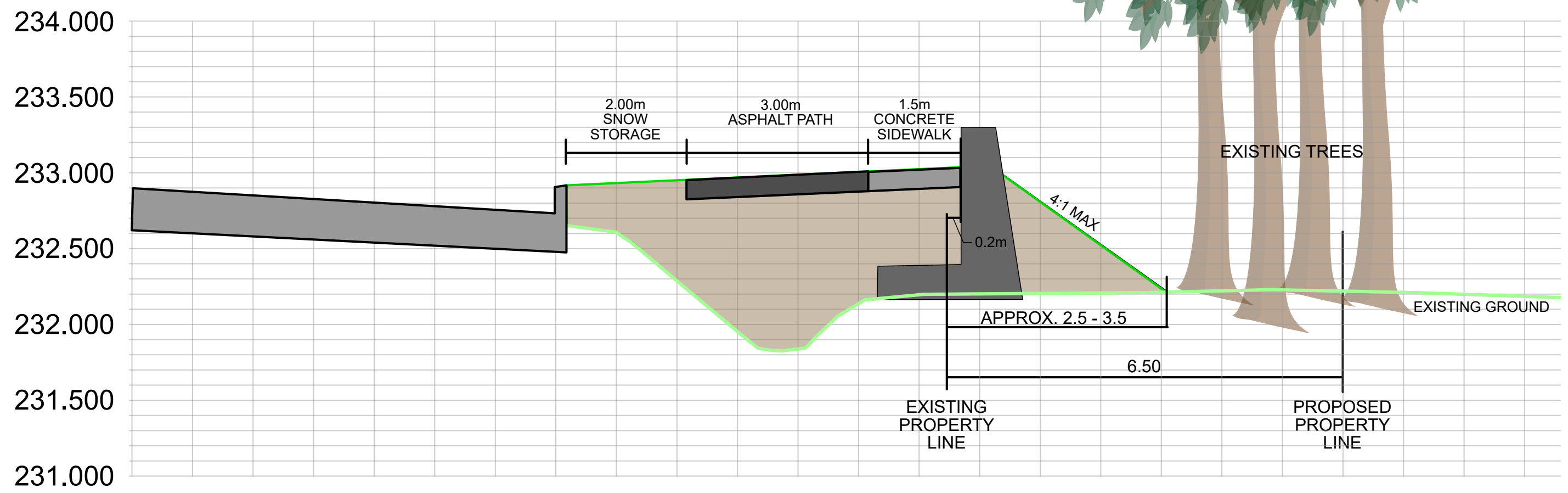
Cross section between proposed intersections
