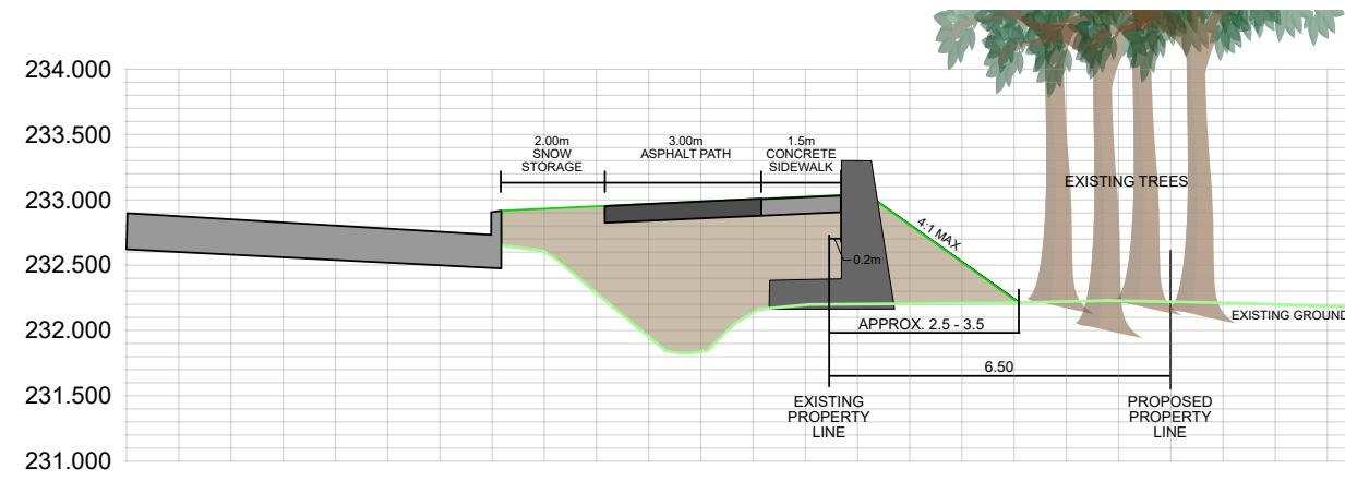
Cross section between proposed intersections
