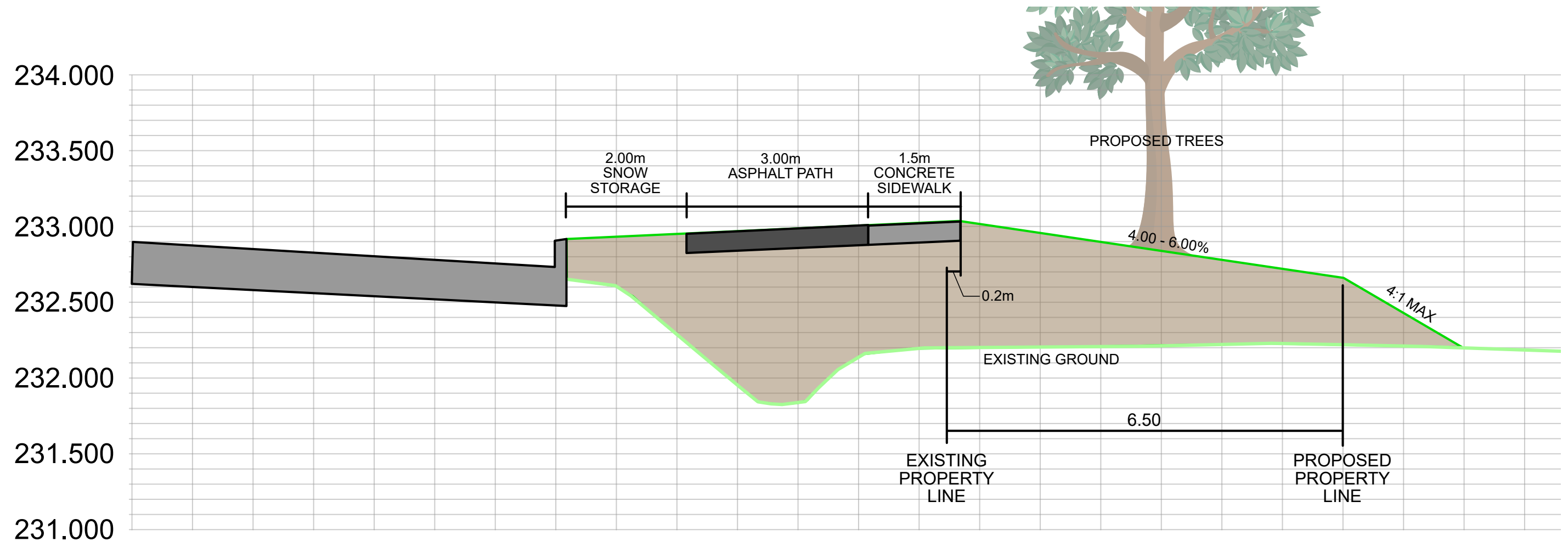
Proposed typical cross section
