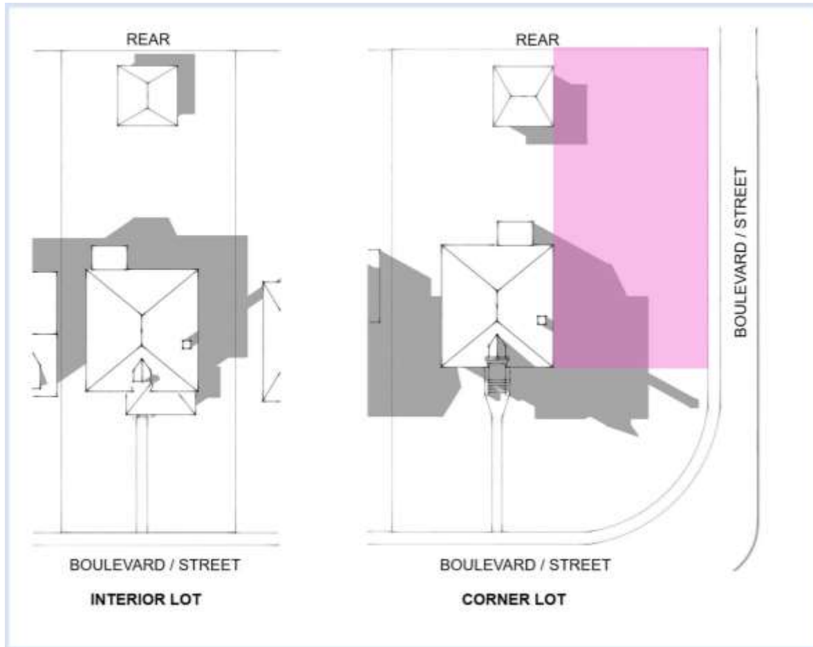
Figure 16: Restricted locations diagram for corner-side yard fences.
