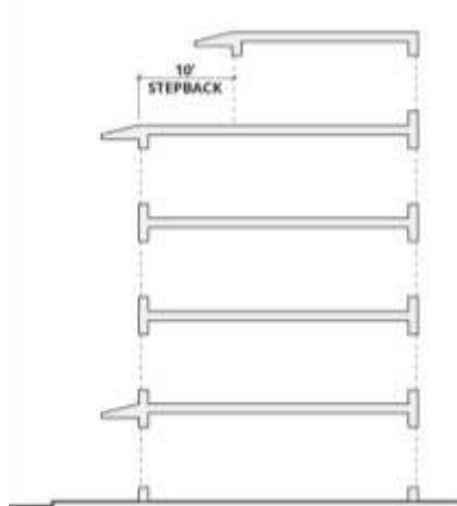
Illustration 1: Fourth Storey Stepback
