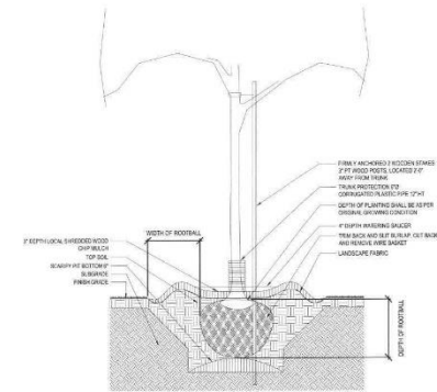
1 TYPICAL TREE PLANTING DETAIL 1/2" = 1'-0"
