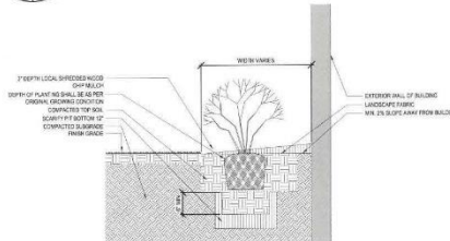
4 SHRUB BED IN SOFT LANDSCAPE 1/2" = 1'-0"
