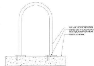
6 TYPICAL BICYCLE RACK 1/2" = 1'-0"
