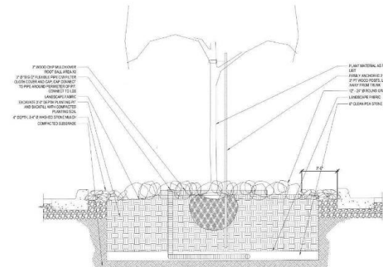
2 TREE PLANTING DETAIL - IN LANDSCAPE BED 1/2" = 1'-0"
