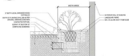
5 SHRUB BED IN CONC SIDEWALK 1/2" = 1'-0"
