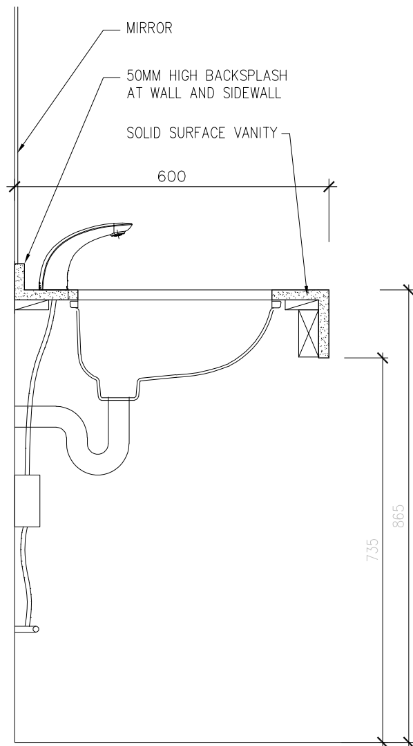
TYPICAL SECTION
