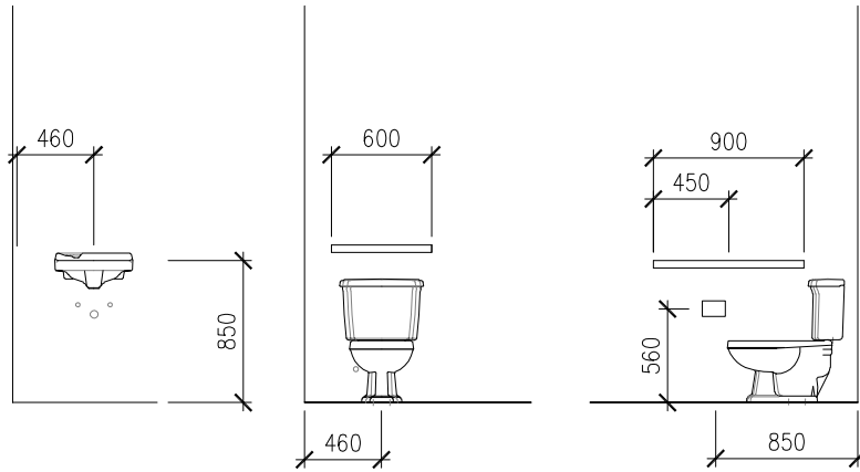
ACCESSORY AND FIXTURE MOUNTING LOCATIONS
