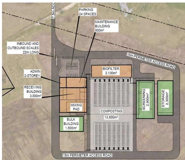
Figure 4 - CASP Conceptual Composting Facility
