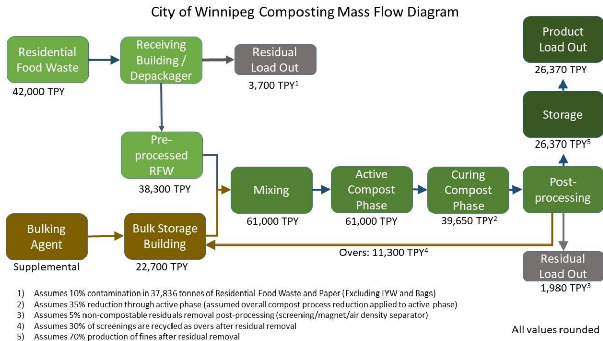
Figure 3 - Mass Flow Diagram Estimated for the Conceptual Composting Facility
