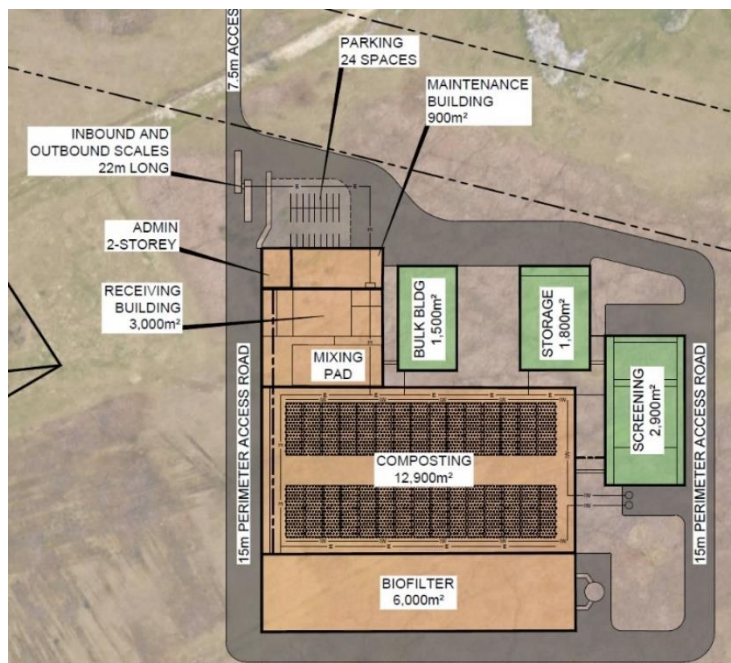
Figure 5 - In-Vessel Conceptual Composting Facility
