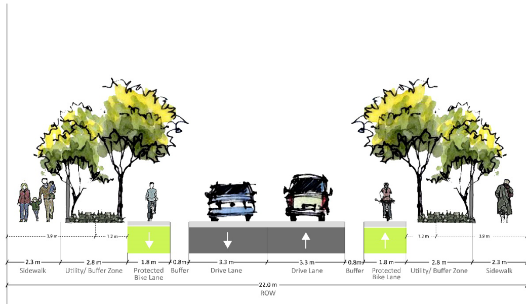
Figure 4.1 – Minor Collector Type A
