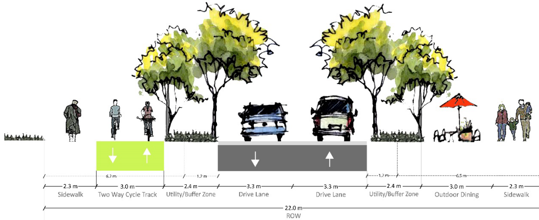
Figure 4.3 – Minor Collector Type B with Outdoor Seating
