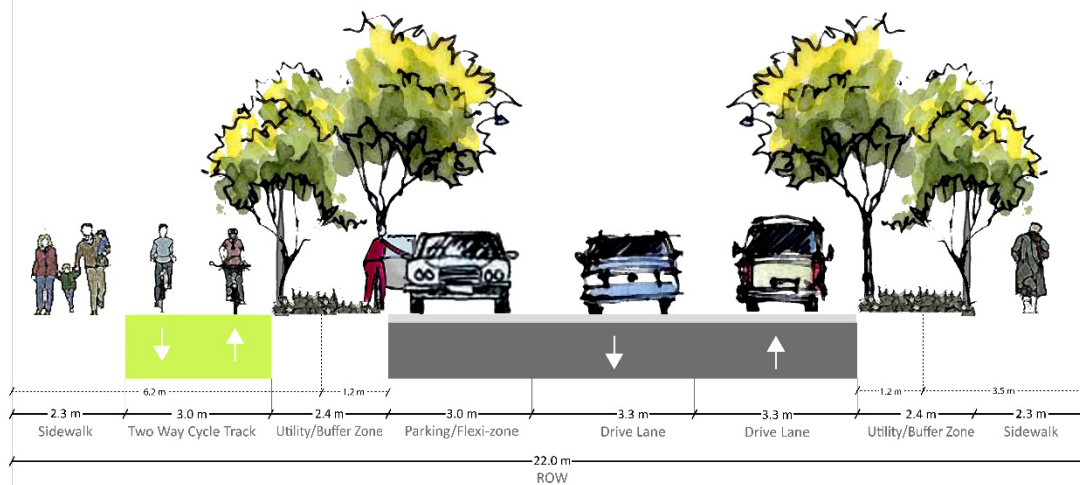
Figure 4.4 – Minor Collector Type B Section with Parking
