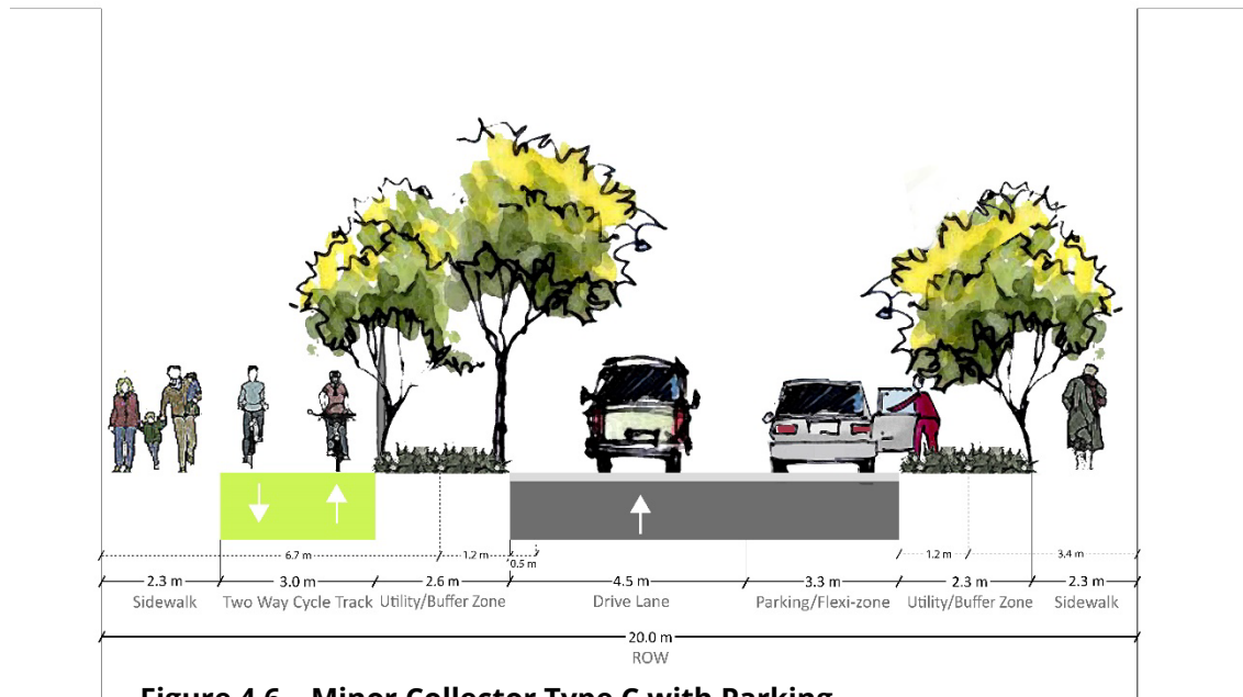
Figure 4.6 – Minor Collector Type C with Parking
