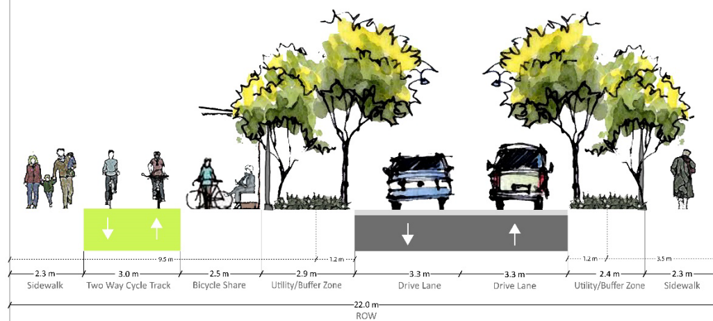
Figure 4.5 – Minor Collector Type B with a Bike Share Station
