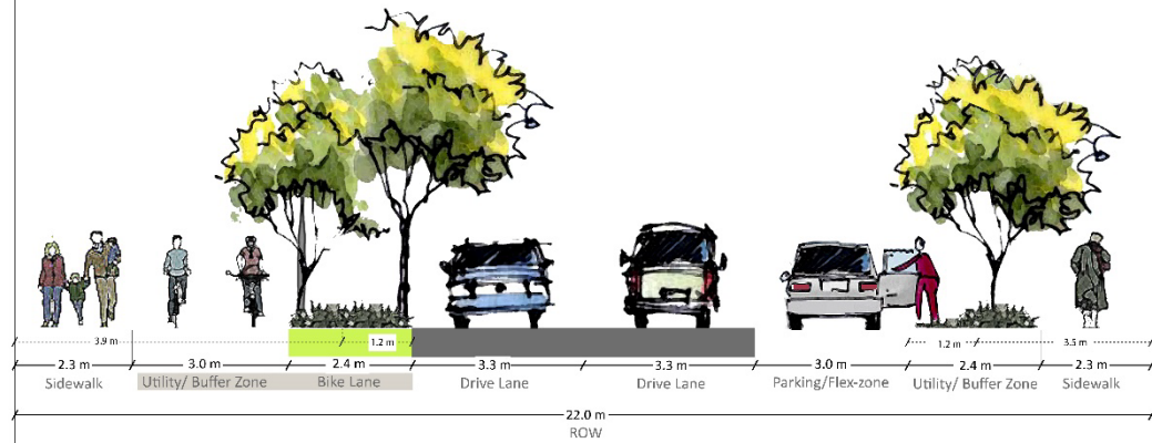
Figure 4.2 – Minor Collector Type B
