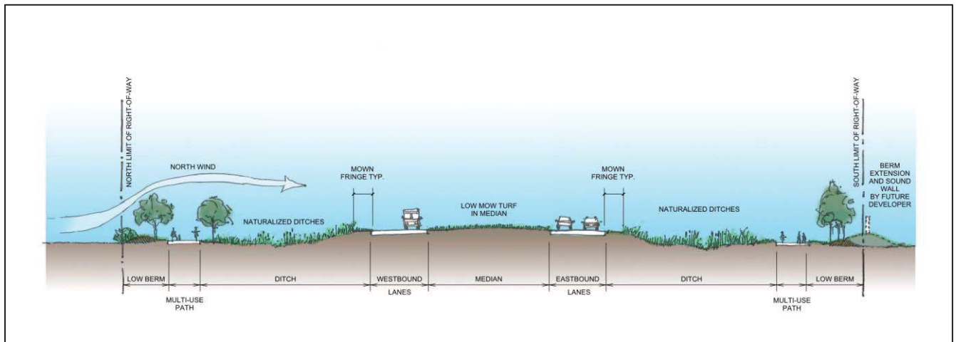
Figure 3.2: Section through Corridor Showing Planting and Landform Strategies
