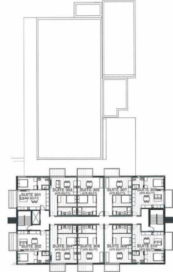
4 FLOOR PLAN (TYPICAL FLOORS 6-15) Scale: 1:200
