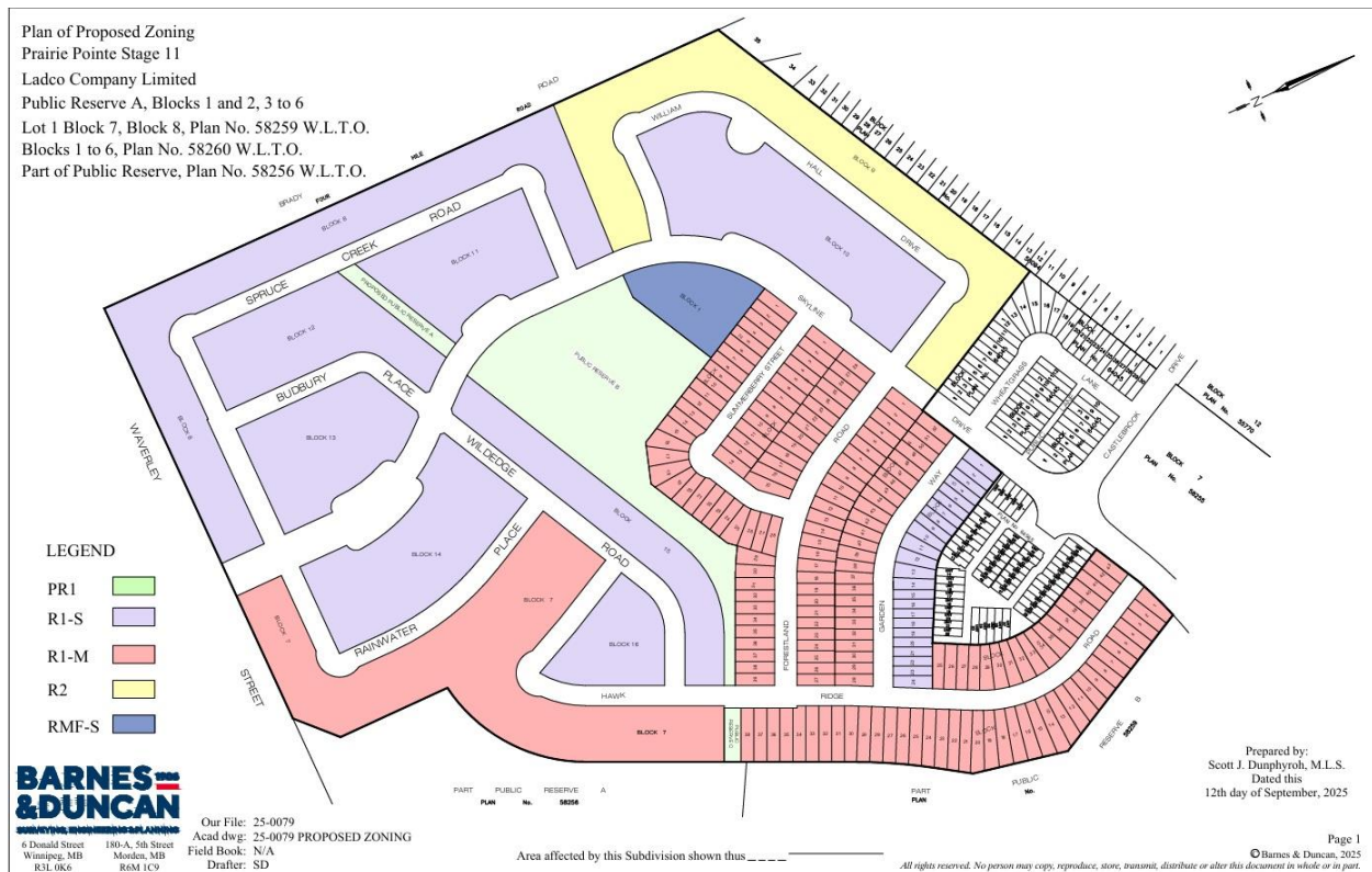
Figure 3: Surveyor's Plan showing proposed lots and public roads on the subject site.
