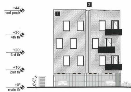
South Elevation
