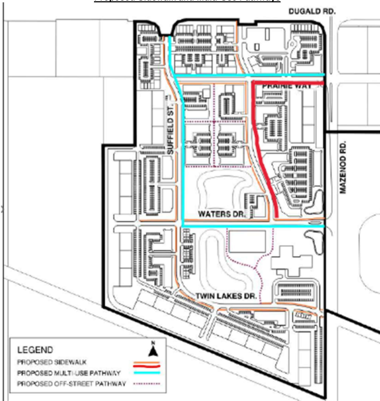
Figure 7.5: Proposed Internal Development Sidewalks and Multi-use Paths
