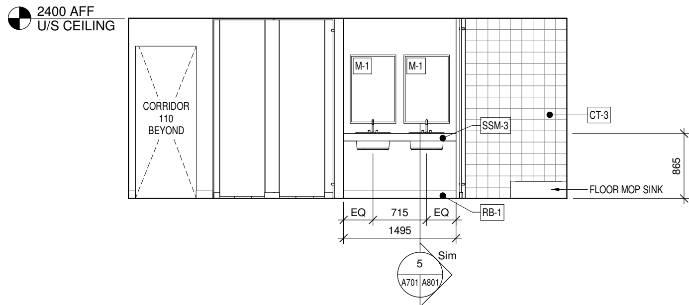
1 Washroom 109 - West A104/A702 1:50
