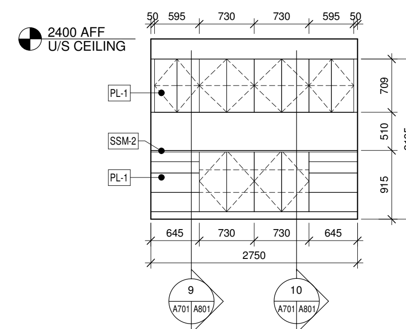
3 Gallery 104 - West A104 A701 1:50
