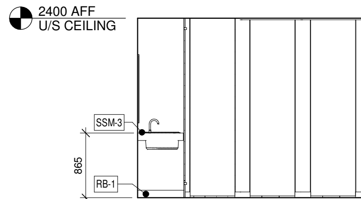
2 UTR 107 - East A104/A702 1:50
