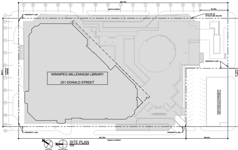
Figure 1: Site Plan for Millennium Library Parkade (grey shading) and Millennium Library
